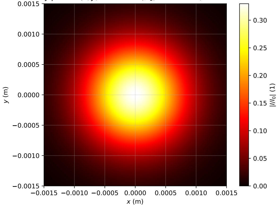
Intensity profile I(x, y, z = 3.981m)/I_0 , P_{in}=0.4P_{cr} , artificial time
